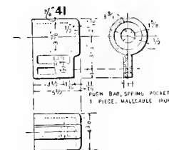
Figs. 1410-1412. Push-bar Spring-pocket.
